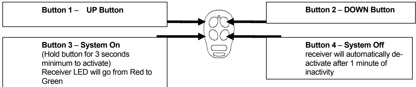
Figure 2 -transmitter
